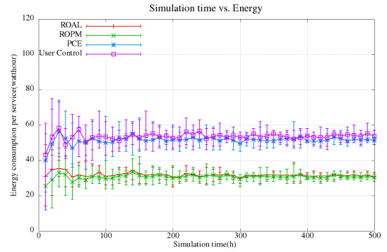
Fig. 8. Energy consumption per service by increasing simulation duration
